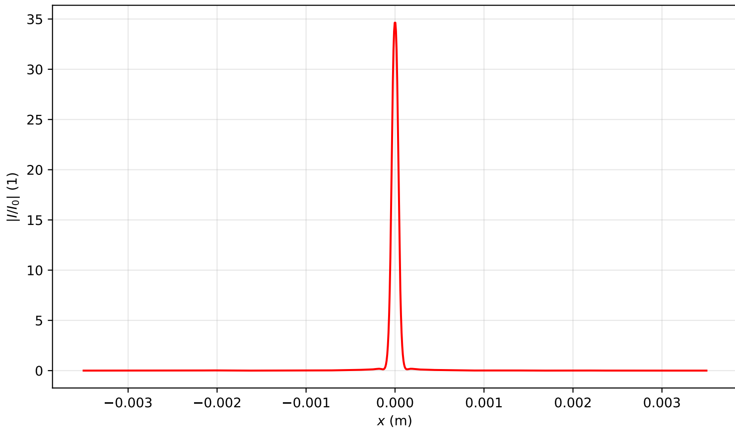
Intensity profile I(x, y = 0, z = 2.866)/I_0 , P_{in}=3.0P_{cr} , artificial time
